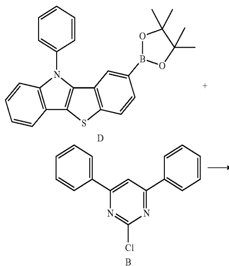
Reaction Scheme 3
