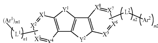
Chemical Formula 1
