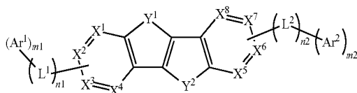
Chemical Formula 1
