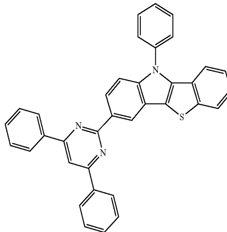
Chemical Formula X-15
