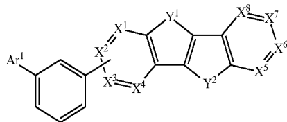
Chemical Formula 4
