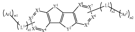
Chemical Formula 1
