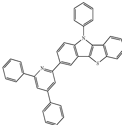
Chemical Formula X-13
