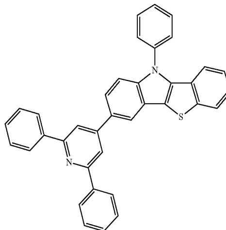
Chemical Formula X-14
