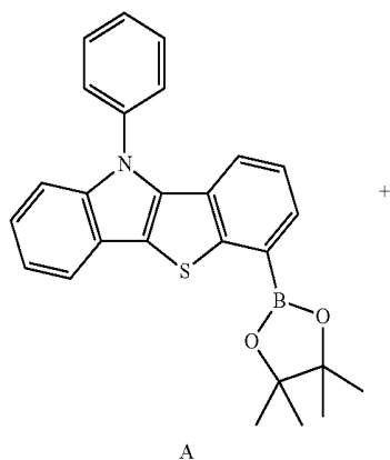
Reaction Scheme 2
