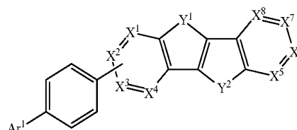
Chemical Formula 3
