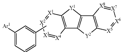
Chemical Formula 4
