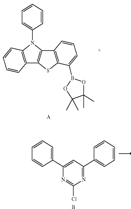
Reaction Scheme 1
