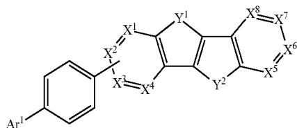
Chemical Formula 3
